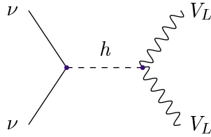
Figure 4.2: Additional diagram involving the exchange of a Higgs boson that contributes to the amplitude for \nu\nu \rightarrow V_L V_L . This diagram cancels the term that grows with energy resulting from the diagrams in Fig. 4.1 if V = W , but not if V = Z .
