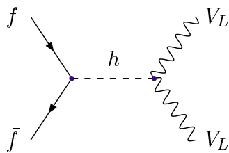
Figure 3.3: Additional diagram involving the exchange of a Higgs boson that contributes to the amplitude for f\bar{f} \rightarrow V_L V_L . This diagram cancels the terms that grow with energy resulting from the diagrams in Fig. 3.1.
