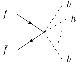
Figure 5.1: Feynman diagram for the interaction of a fermion with n Higgs bosons.
