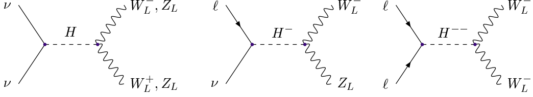
Figure 4.4: Additional diagrams that contribute when the Majorana neutrino acquires its mass via a coupling to an SU(2)_L -triplet Higgs \bar{\text{eld}} .
