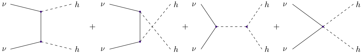
Figure 4.3: Feynman diagrams that contribute to the amplitude for \nu\nu \rightarrow hh . Only the last diagram grows with energy.
