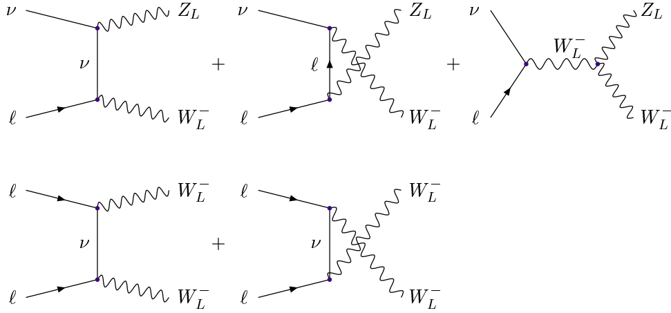
Figure B.1: Feynman diagrams that contribute to the amplitude for \nu \bar{\ell} \rightarrow \ell \nu ! W_L^i Z_L and W_L^i W_L^i in unitary gauge.
