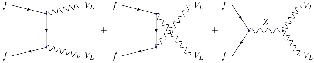
Figure 3.1: Feynman diagrams that contribute to the amplitude for f\bar{f} \rightarrow V_L V_L in unitary gauge. The middle diagram is absent if V = W ; the last diagram is absent if V = Z .
