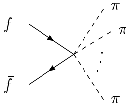
Figure 3.2: Feynman diagram for the interaction of a fermion with n Goldstone bosons.
