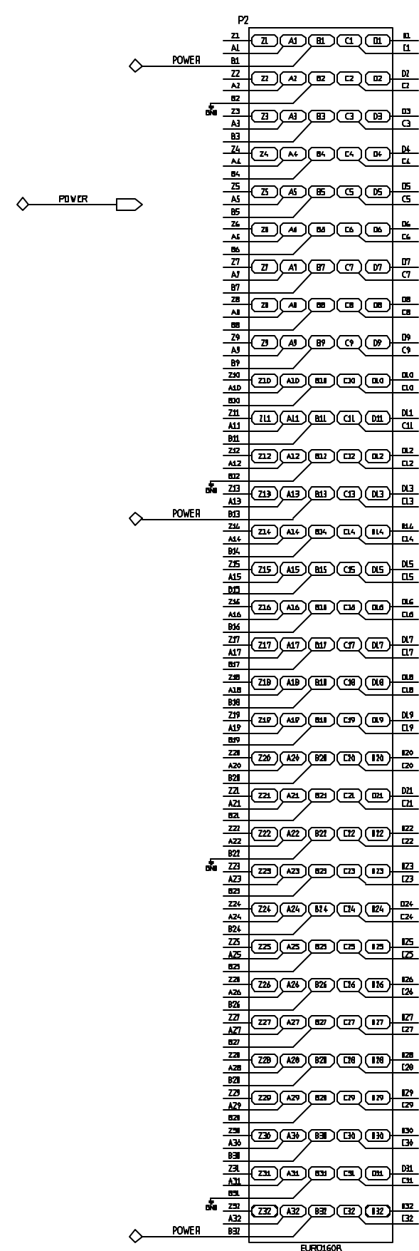
P2 VME Connector
