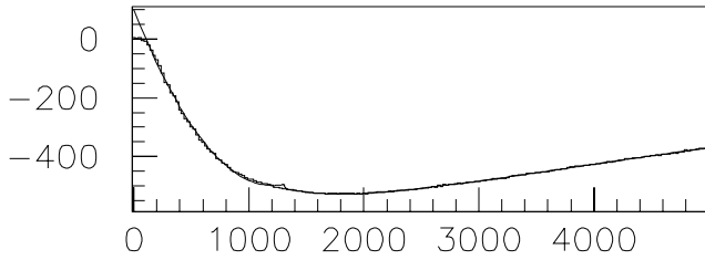
236 ch. 2 (mV, nsec).. mixer-shaper..in
