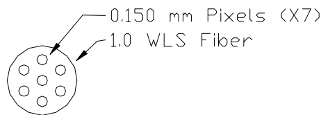
Figure 1 Seven-GPD pixel layout to match a 1.0 mm diameter WLS fiber footprint.
